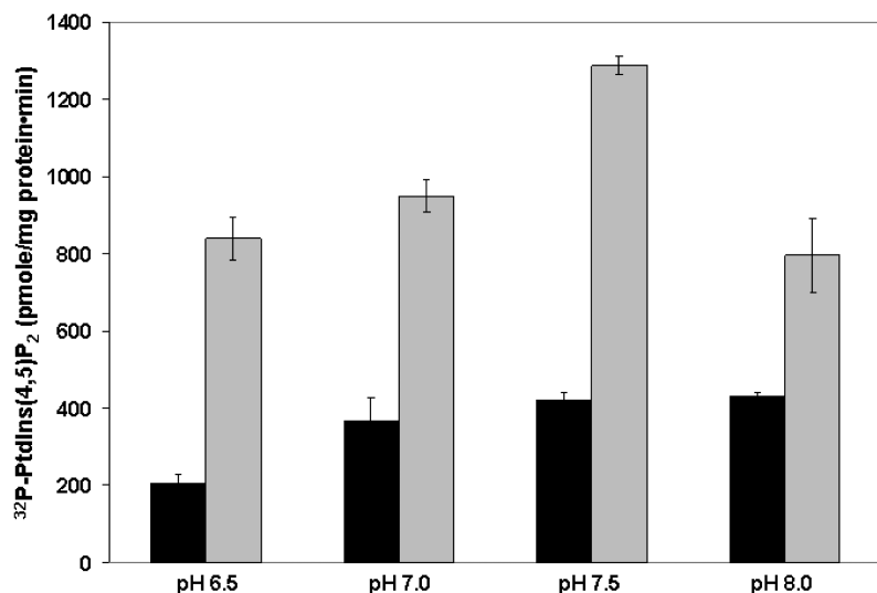
Fig. 4. Purified recombinant GST- AIP1K1 (10 \mu g) was assayed with 125 \mu M PtdIns4P prepared by sonication (black bars) or in 5 mM \beta CD (gray bars) at various pH values. Data are averages of two independent experiments.
